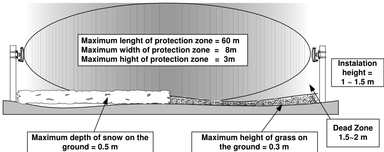
Fig.1. Installation and Protection zone
