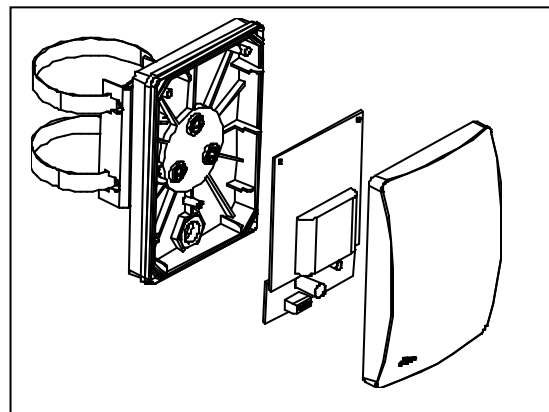
Fig. 8. CSB-60T - Transmitter unit with binding band.
