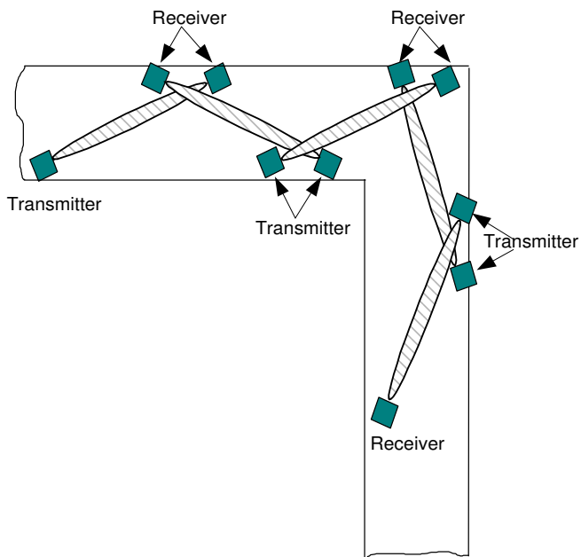
Fig. 3. Overlapping Installation of multiple CSB-60 systems.
